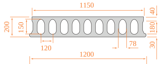
200mm deep Hollowcore slab
