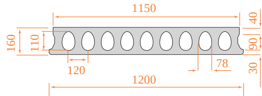
160mm deep Hollowcore slab
