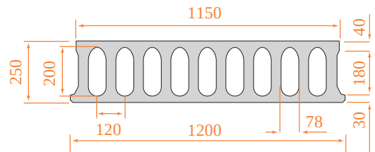
250mm deep Hollowcore slab
